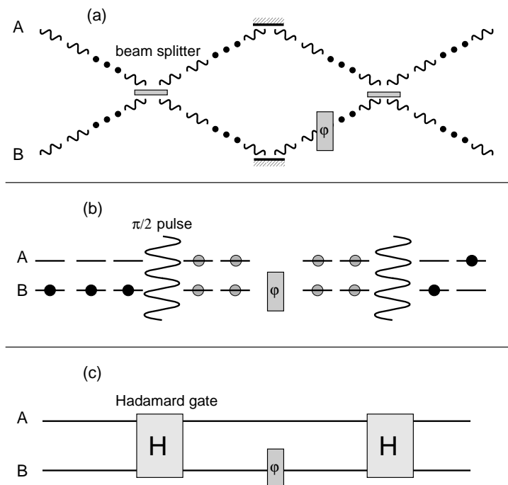
Figure 2. Three distinct representations of phase measurement: (a) a Mach-Zehnder interferometer, (b) Ramsey spectroscopy, and (c) a generic quantum logic gate. The two basis states of a qubit, |0\rangle and |1\rangle , may be regarded as the atomic two levels, or the two paths in a Mach-Zehnder interferometer. The state |\varphi\rangle can be regarded as a single photon state just before the second beam splitter in the Mach-Zehnder interferometer, or the single atom state just before the last \pi/2 -pulse in the Ramsey interferometer.
