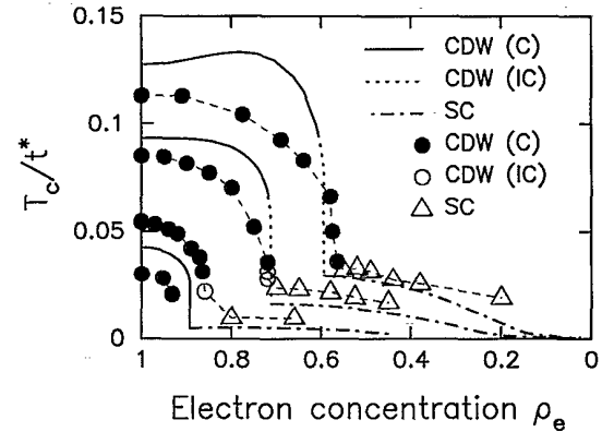
FIG. 2. Phase diagram for the Holstein-Hubbard model with g = 0.5 , \Omega = 0.5 , U = -1.0 , and U_C = 0.0, 0.25, 0.5 , and 0.75 . The solid dots (lines) are for the commensurate CDW, the open dots (dotted lines) are for the incommensurate CDW, and the open triangles (dot-dashed lines) are for the SC as determined from a QMC (IPT) calculation. There are no transitions detected by the IPT for U_C = 0.75 . The dashed line through the QMC points is a guide to the eye.
