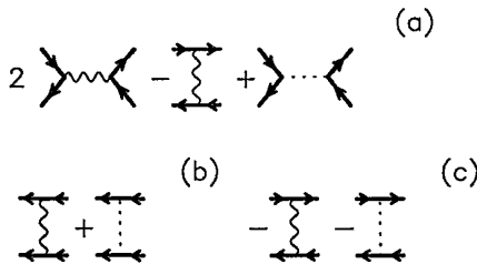
FIG. 1. Lowest-order contribution to the irreducible vertex function in the (a) charge-density-wave, (b) superconducting, and (c) spin-density-wave channels. The solid lines denote electron propagators, the wiggly lines denote phonon propagators, and the dotted lines denote the Coulomb repulsion.
