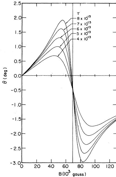
FIG. 1. Plot of the Faraday rotation \theta vs the magnetic field B . The parameters used are N = 2.3 \times 10^{12} \text{ cm}^{-2} , m^* = 0.19m_e , where m_e is the rest electron mass, n_o = 1.95 , n_s = 3.44 , \omega = 6.455 \times 10^{12} \text{ s}^{-1} , and for the \tau values indicated on the curves. The vertical line corresponds to the value \omega = \omega_c or B = 6.97 \times 10^4 \text{ G} .
