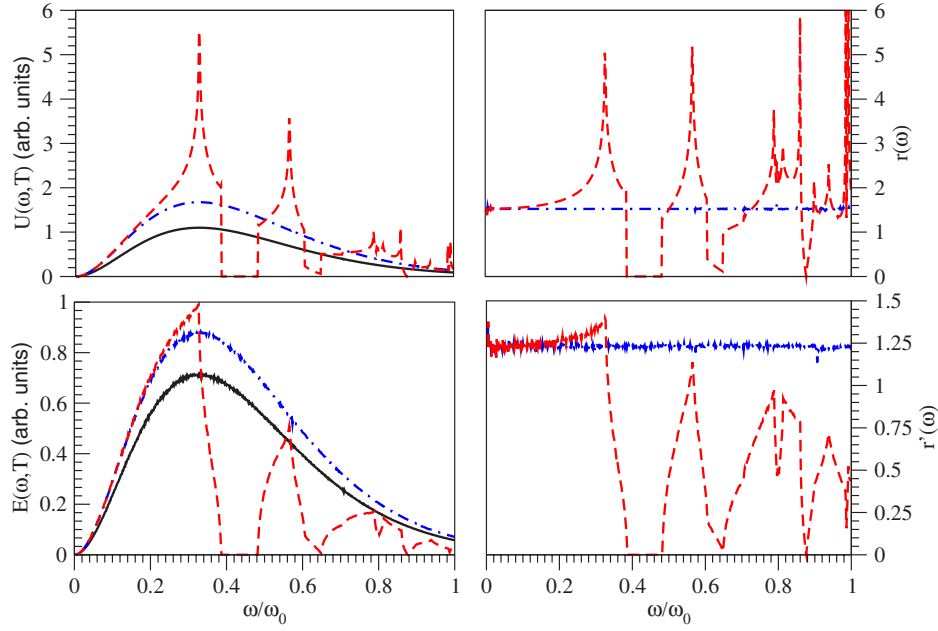
FIG. 1. (Color online) Frequency dependence of the spectral energy density (left-hand panel, upper figure) and spectral hemispherical emissive power (left-hand panel, lower figure) for free space (continuous line), a homogeneous dielectric with dielectric constant equal to \epsilon=1.52 (dotted-dashed line) and the model photonic crystal (see text; with a long wavelength effective dielectric constant \epsilon_{av}=1.52 ) (dashed line). The temperature is chosen such that the conventional blackbody exhibits a maximum at the frequency of the first van Hove singularity of the model system's DOS, \omega_{max} \approx 0.327\omega_0 , and frequencies are measured in units of \omega_0=2\pi c/a . On the right-hand panel, we show the ratios of the respective quantities relative to their free space values.
