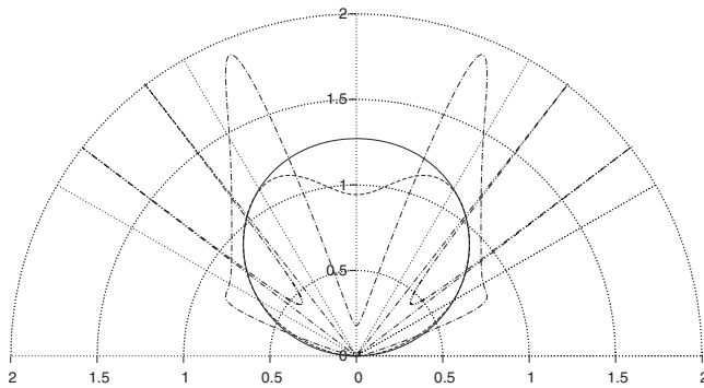
FIG. 3. Dependence of the directional spectral emissive power within the 2D model photonic crystal on the emission angle for \omega_1/\omega_0=0.25 (continuous line), \omega_2/\omega_0=0.31 (dashed line), \omega_3/\omega_0=0.327 (dotted-dashed line), and \omega_5/\omega_0=0.34 (double dotted-dashed line). For visualization purposes the first three quantities are multiplied by a factor of 3.
