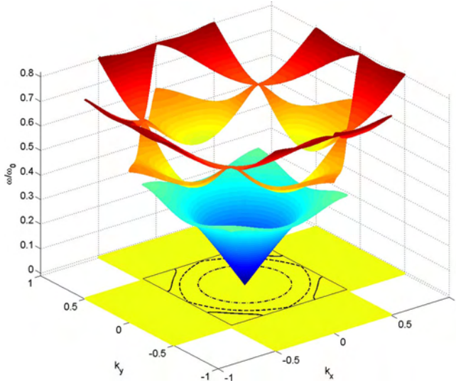
FIG. 2. (Color online) Band structure for a 2D square lattice of dielectric cylinders ( \epsilon=8.41 , r/a=0.15 ) in air. In the \omega=0 plane we show the \mathbf{k} -space domain used (first three Brillouin zones) and the isofrequency contours for \omega/\omega_0=0.25 (dotted-dashed line), 0.327 (line), 0.345 (continuous line).
